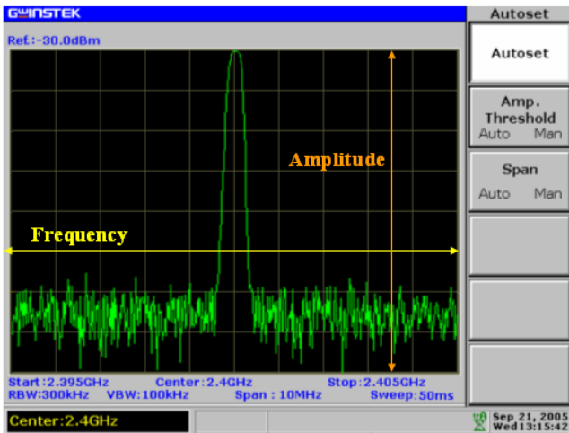
Fig. 8. Using these parameter settings including frequency, span per division and reference level, it is possible to make a variety of measurements using only the primary controls
